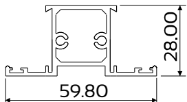
DIE No. W52697 Cas28 Mullion 28mm Standard
