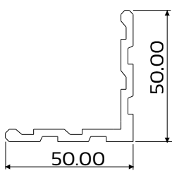
DIE No. W52695 Cas28 Corner Cleat 50mm
