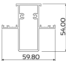
DIE No. W54348 Cas28 Mullion 54mm
