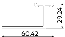
DIE No. W24052 Cas28 Fixing Lug Twist In
