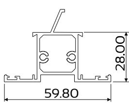
DIE No. W13142 Cas28 Mullion 28mm W/Bar
