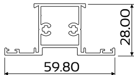
DIE No. W55683 Cas28 Mullion 28mm
