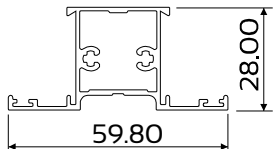
DIE No. W50957 Cas28 Mullion 28mm Econo
