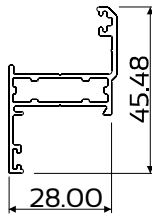
DIE No. W55497 Cas28 Picture Frame Sash
