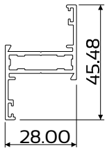
DIE No. W55682 Cas28 Sash Tubular
