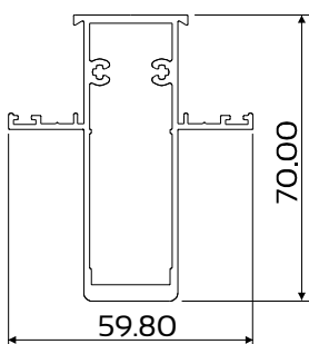
DIE No. W54329 Cas28 Mullion 70mm
