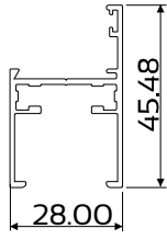
DIE No. W32026 Cas28 Frame 28mm Equal Leg
