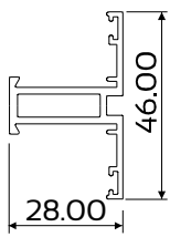
DIE No. W53283 Cas28 Mullion 28mm Cottage Pane
