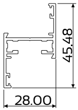
DIE No. W32025 Cas28 Frame 28mm Unequal Leg
