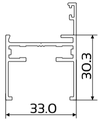
DIE No. W32039 Equal Leg Outer Frame
