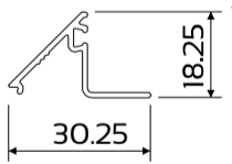
DIE No. W33137 Cas34 Bead Multi 13mm
