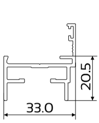
DIE No. W33134 Cas34 Frame 34mm Short Leg
