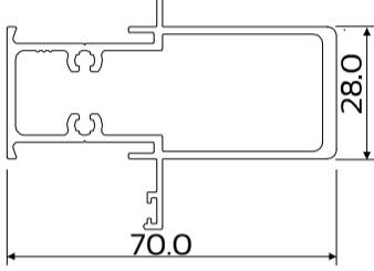
DIE No. W56270 Cas34 70mm Mullion
