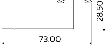
DIE No. W10627 Fixing Lug
