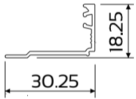
DIE No. W33136 Cas34 Bead Double Glaze
