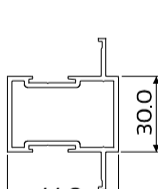
DIE No. W53033 Midrail Glazing Bar
