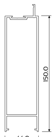
DIE No. W44094 Head/Sill Rail R6
