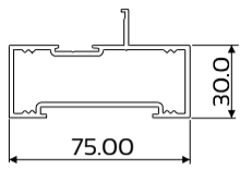
DIE No. W44084 Frame Rec Back 75mm 26B
