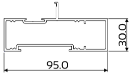
DIE No. W55365 Frame Rec Back 95mm
