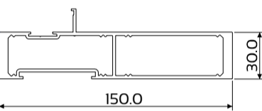
DIE No. W55362 Frame Rec Back 150mm
