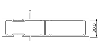
DIE No. W54043 H/D Mullion 150mm
