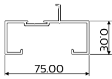
DIE No. W26154 Frame Open Back 75mm 26C
