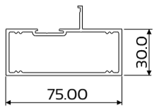
DIE No. W53194 Frame Flat Back 75mm 26E
