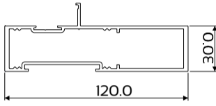
DIE No. W55363 Frame Rec Back 120mm
