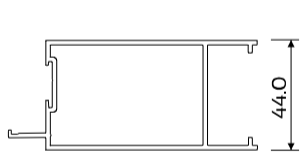
DIE No. W44088 Head/Sill Rail R4
