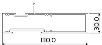
DIE No. W56084 Frame Rec Back 130mm
