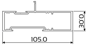
DIE No. W55364 Frame Rec Back 105mm
